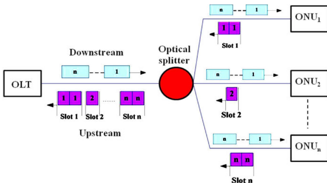
Figure 2.5: GPON Architecture [1]
