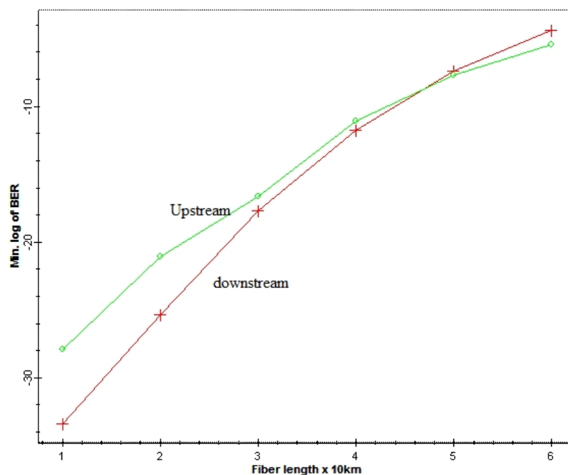
Figure 4.25: BER of PSK for system of varied fiber length
